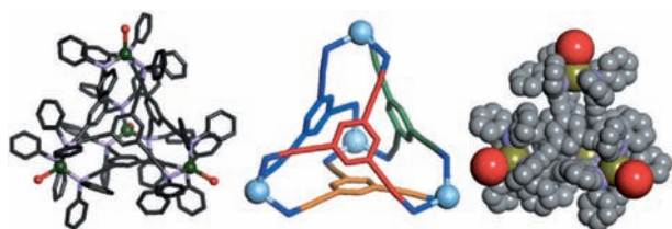
Figure 1. Crystal structure of the [M_4(tppeb)_4]_4I_4 clusters. Each cluster is shown in a distinct depiction: the complete [Cu_4(tppeb)_4]_4I_4 cluster is shown as sticks (left); to emphasize the cluster geometry, the [Ag_4(tppeb)_4]_4I_4 cluster is shown with phenyl groups removed and each ligand in a different color (middle); and the [Au_4(tppeb)_4]_4I_4 cluster is shown as a space-filling model (right).
